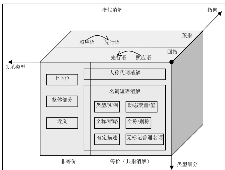
Fig.2 Three dimension concepts relationship related to coreference resolution 图2 共指消解相关概念的三维关系
