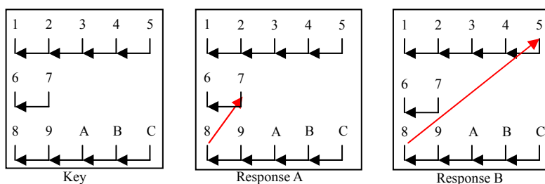
Fig.8 Sketch of the problem in Valain method
