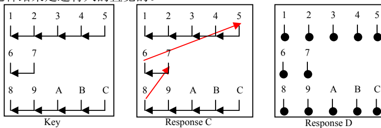
Fig.9 Sketch of the problem in B-CUBED method
