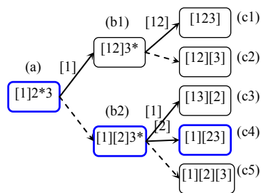
Fig.5 Bell tree for three mentions 图 5 三个 Mention 的 Bell 树
